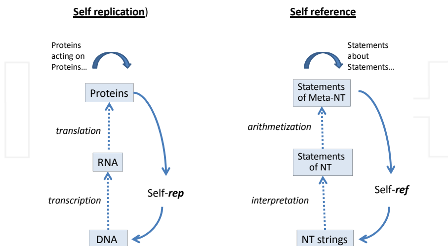
Fig. 6. Hofstadter’s Self-ref and Self-rep
