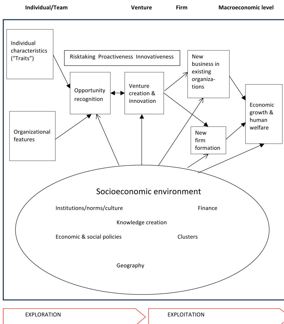
Figure 1. Domain of Entrepreneurship Research
